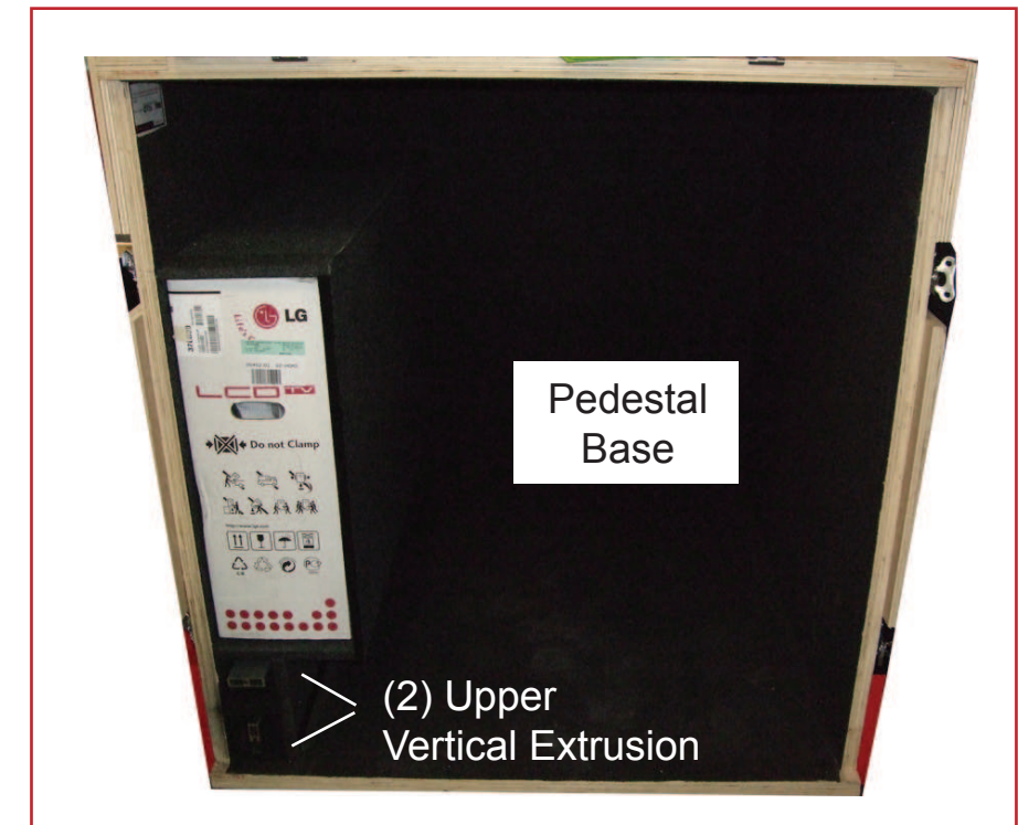
Front View of Crate
