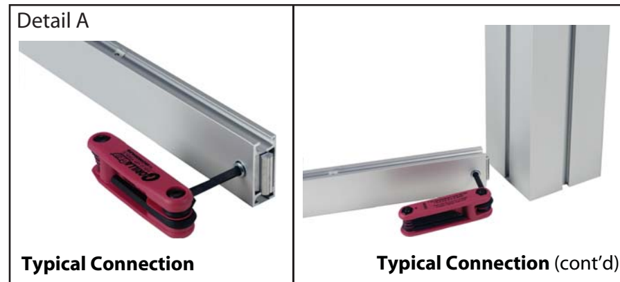
Typical Connection Tightening the lock with the Hex Key Tool expands the lock and creates a strong positive connection.
