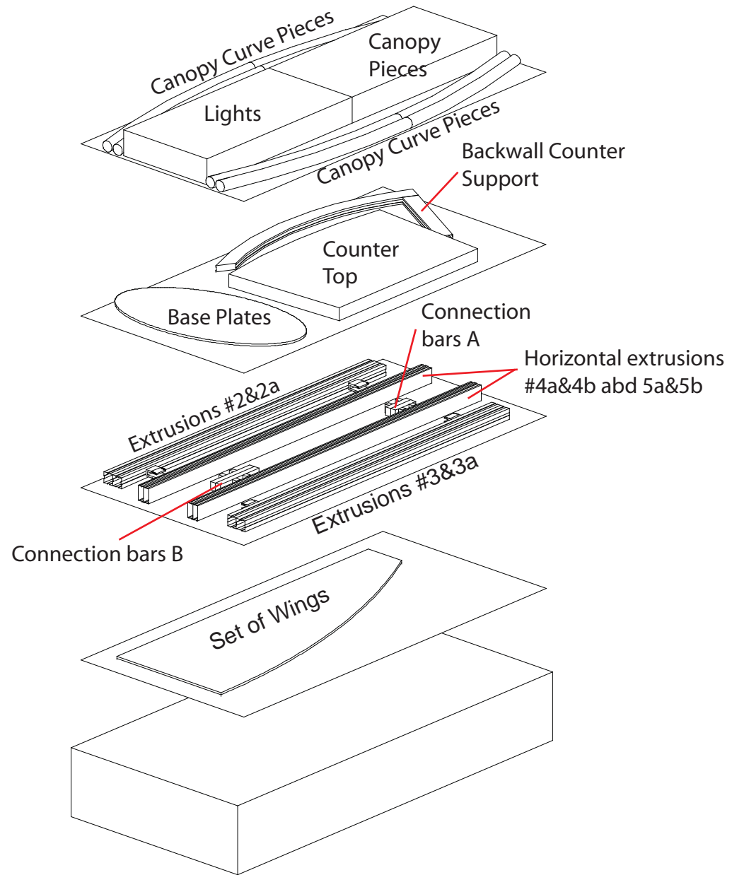
(1) Backwall Components
