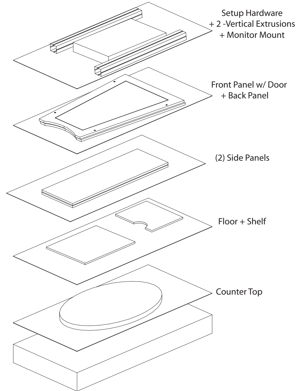
Case 1 - (1) Modified LTK-1001 Pedestal
