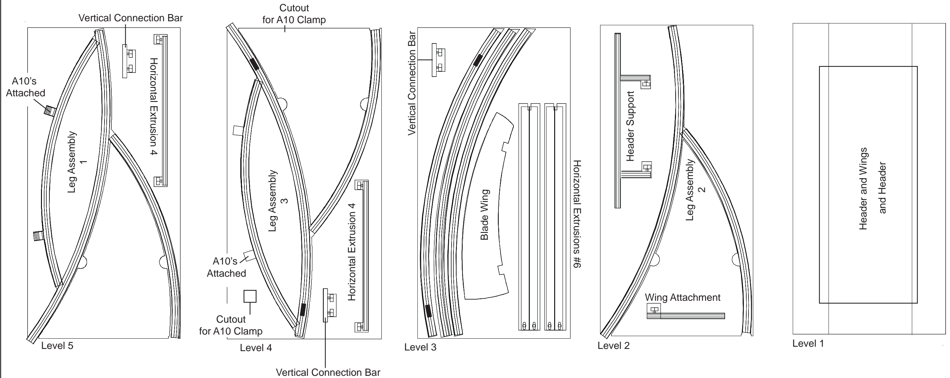
Top View of each Level
