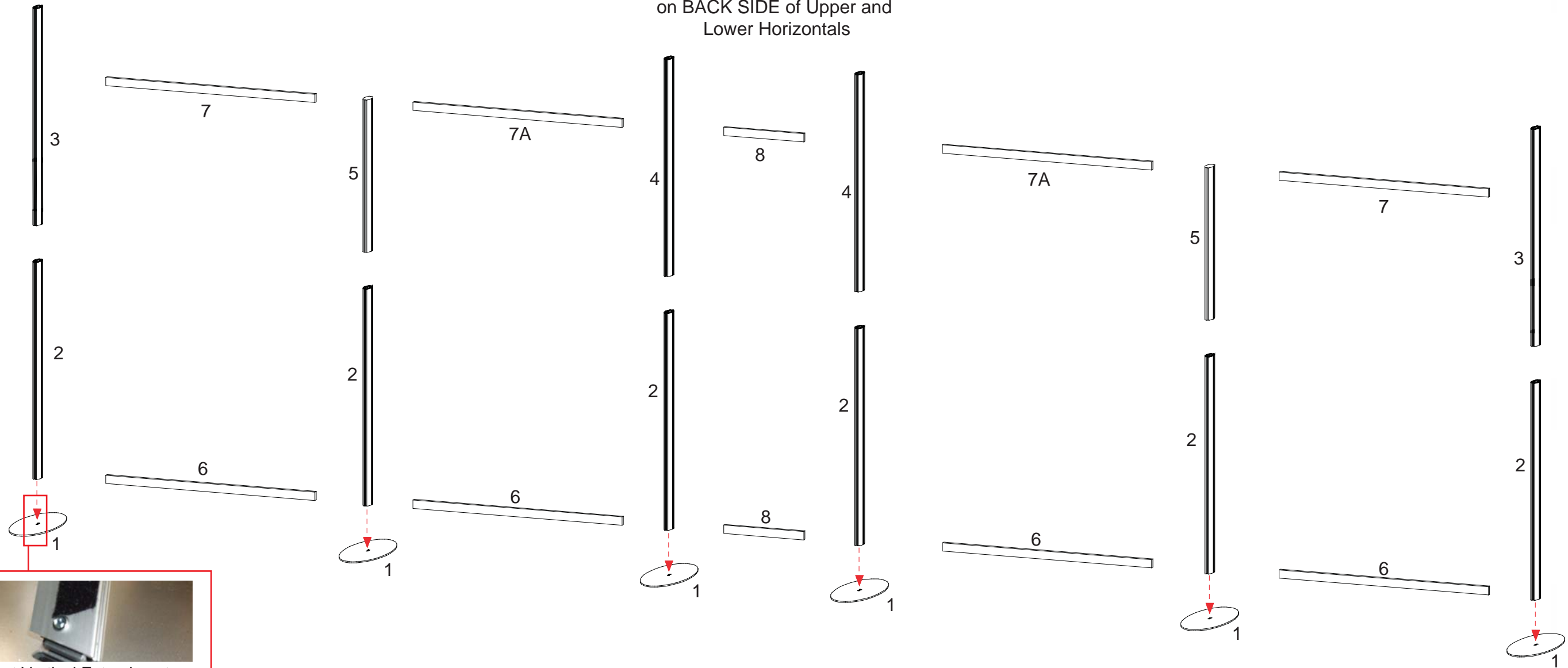
Connect Vertical Extrusions to Base Plates by placing lock into slot and tighten with tool.
