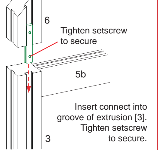
Back View of Backwall
