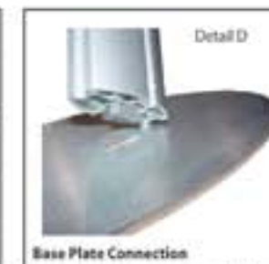
Base Plate Connection
