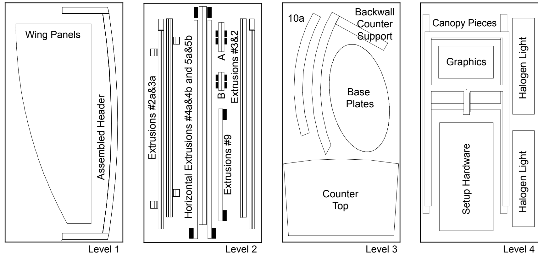
Top View of Each Level
